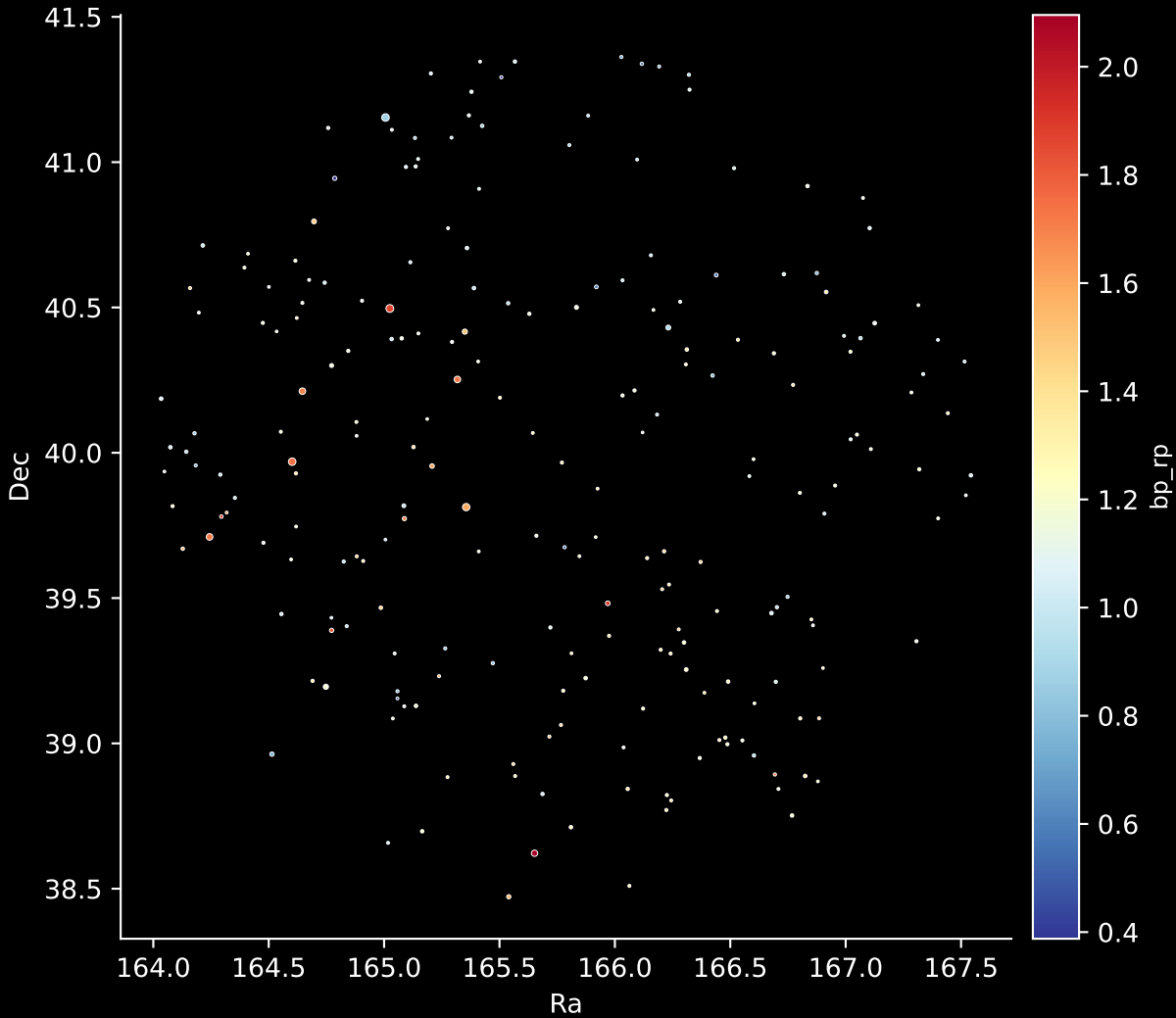
APOGEE DR17 Field: [CA_161-06_btx] Stars: 220
