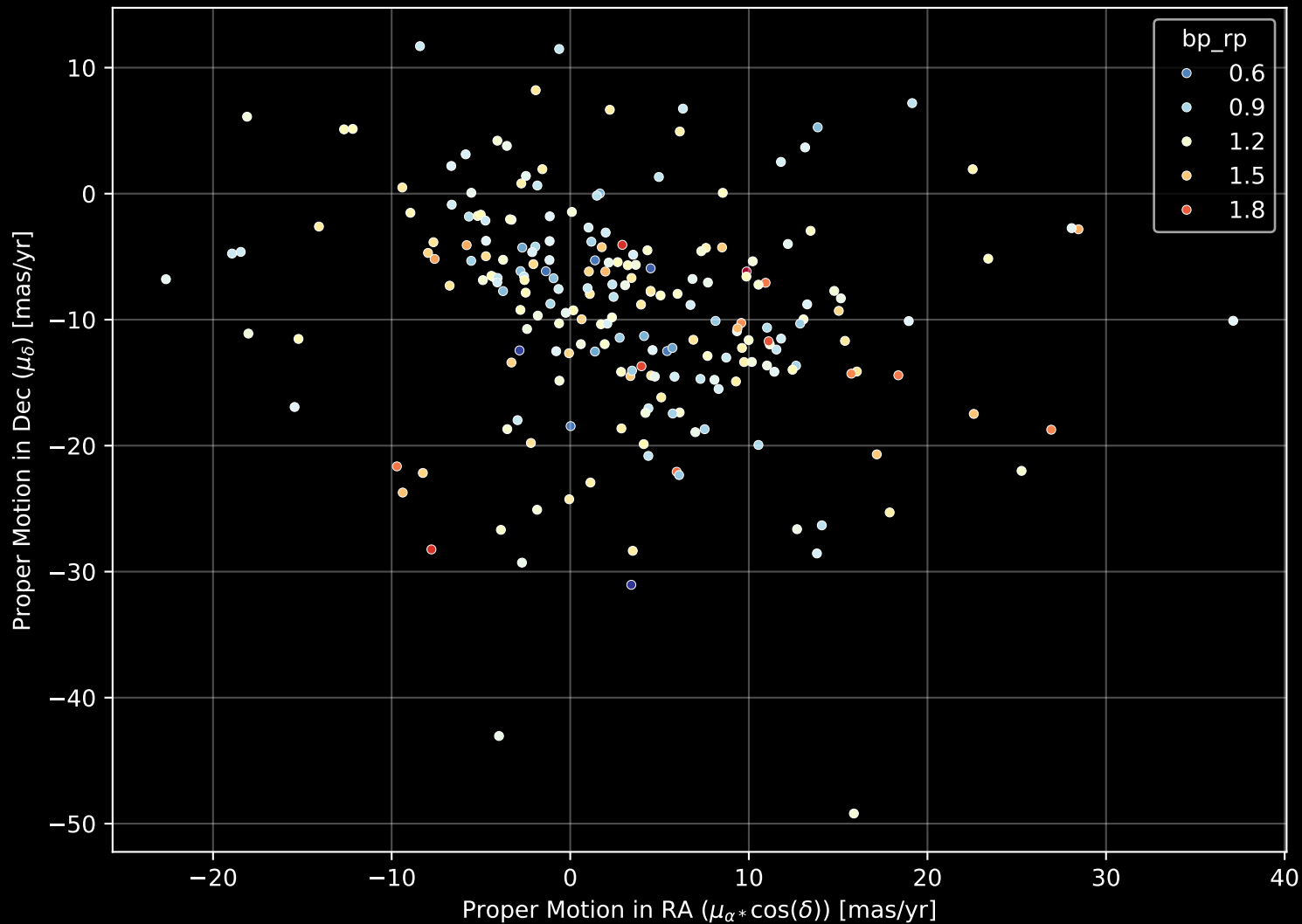
APOGEE DR17 Field: [CA_161-06_btx] Proper Motion Diagram (n= 220)
