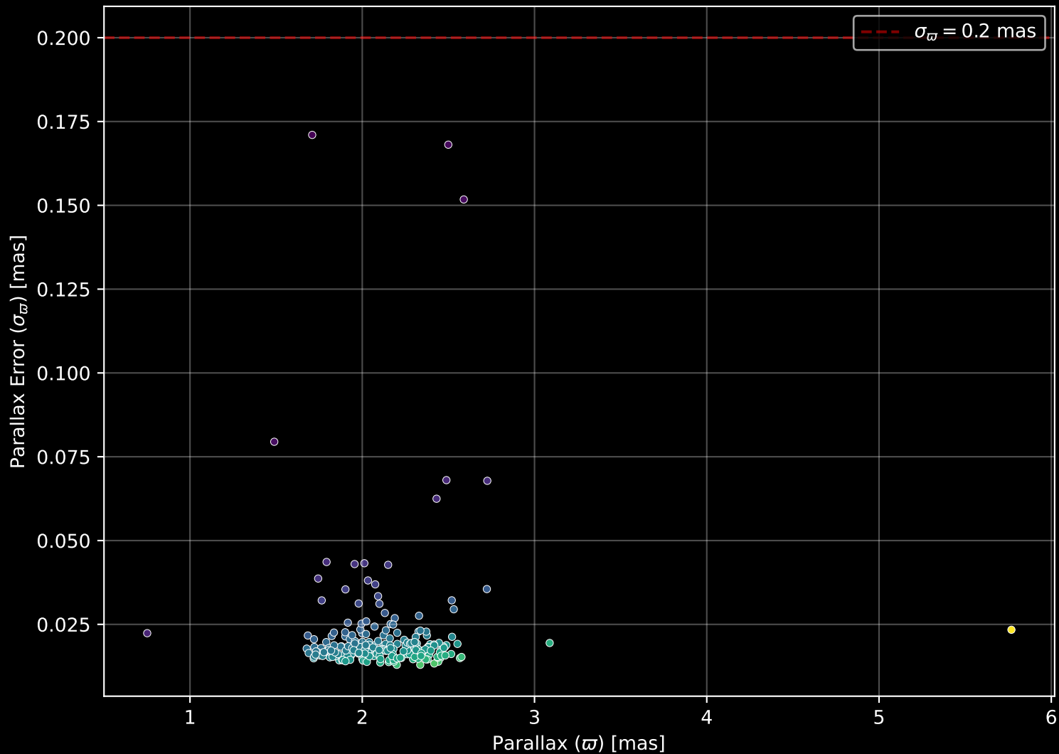
APOGEE DR17 Field: [CA_161-06_btx] Parallax Quality (n= 220)
