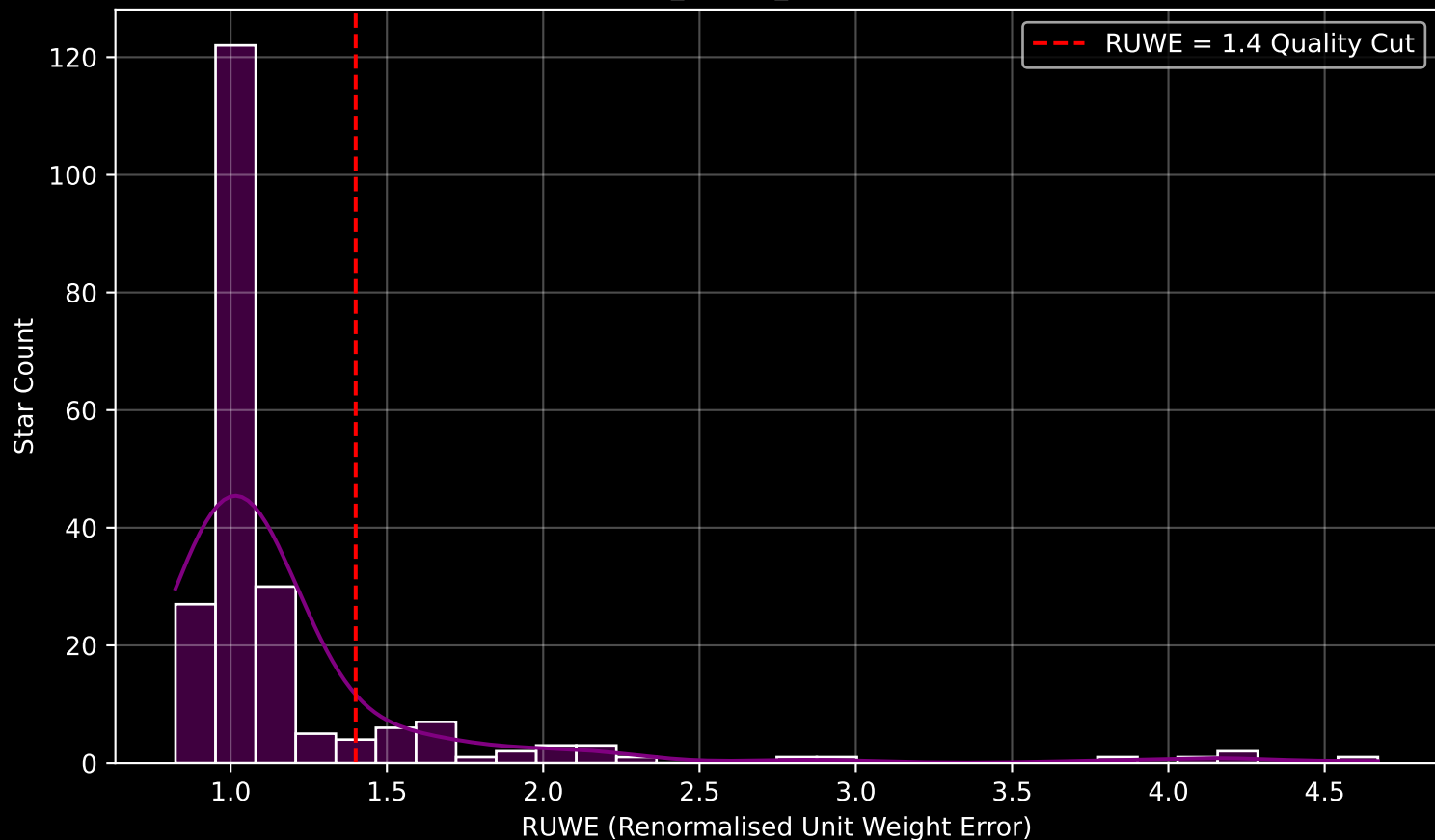
GAPOGEE DR17 Field [CA_161-06_btx] RUWE Distribution (n= 218)
