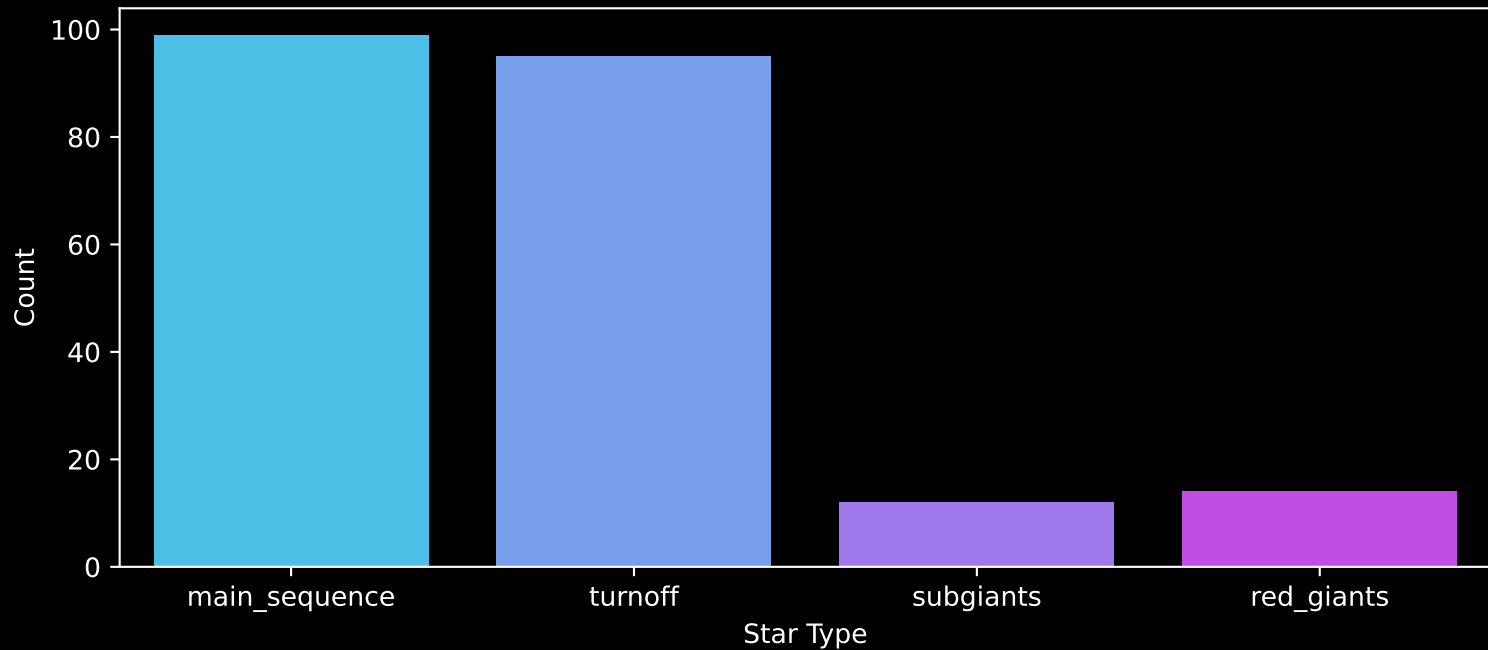
APOGEE DR17 Field: [CA_161-06_btx] Count plot of Star Type
