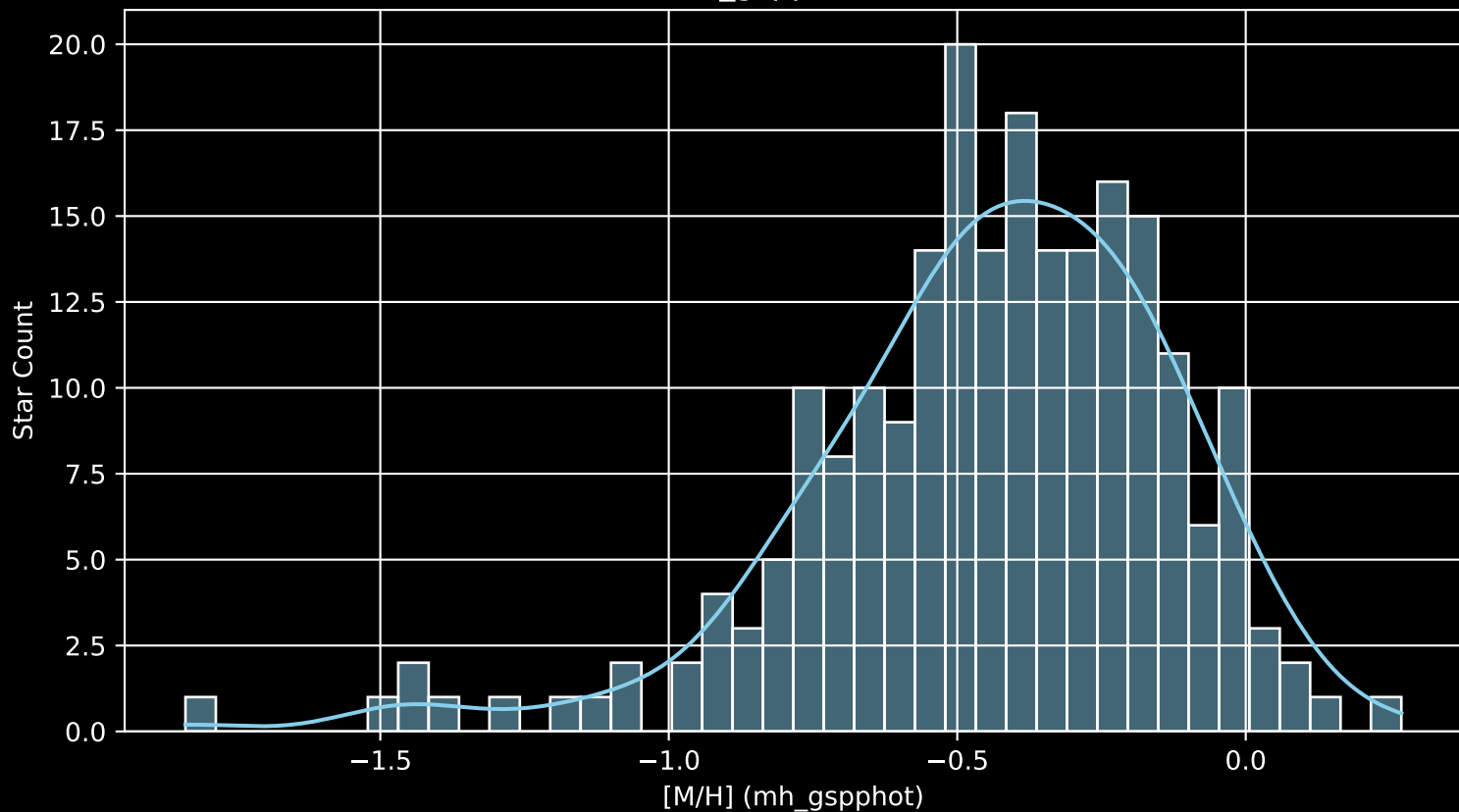
APOGEE DR17 Field: [CA_161-06_btx [M/H] (mh_gspphot) (n= 220)
